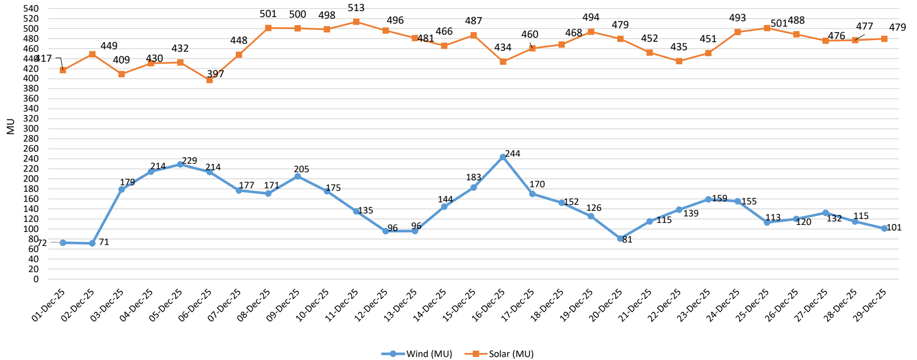
All India Wind & Solar Power Daily Generation Report
