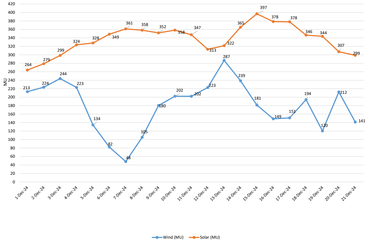
All India Wind & Solar Power Daily Generation Report
